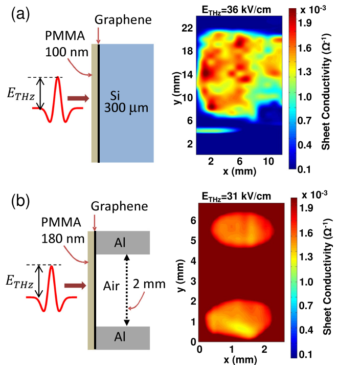
FIG. 1. Sheet conductivity images of (a) PMMA/graphene-on-Si (inhomogeneous) and (b) free-standing PMMA/graphene (homogeneous) samples at low THz intensity ( E_{\text{THz}} \sim 30 kV/cm). Raster images were taken over (a) 25 \times 13 -mm 2 rectangle and (b) two 2-mm diameter holes with (a) 1-mm and (b) 0.2-mm pixel size. In the images, (a) the rectangular area of graphene is colored with cyan, yellow, and red, and (b) the circles of graphene are colored with yellow and orange.
