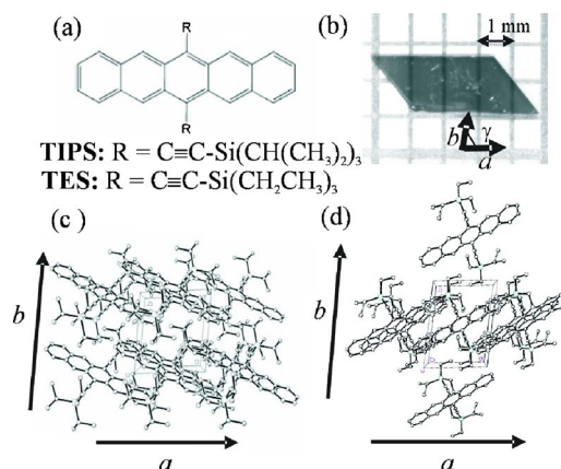
FIG. 1. (a) Molecular structure of TIPS and TES derivatives. (b) Typical TIPS crystal. Molecular packing in (c) TIPS and (d) TES crystals.
