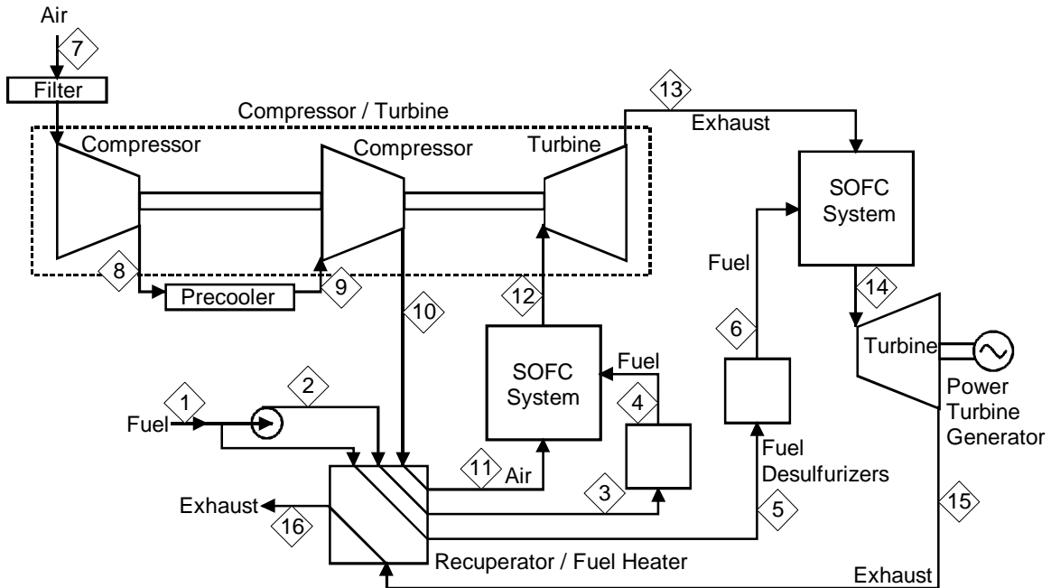
Figure 7-7 Schematic for a 4.5 MW Pressurized SOFC
