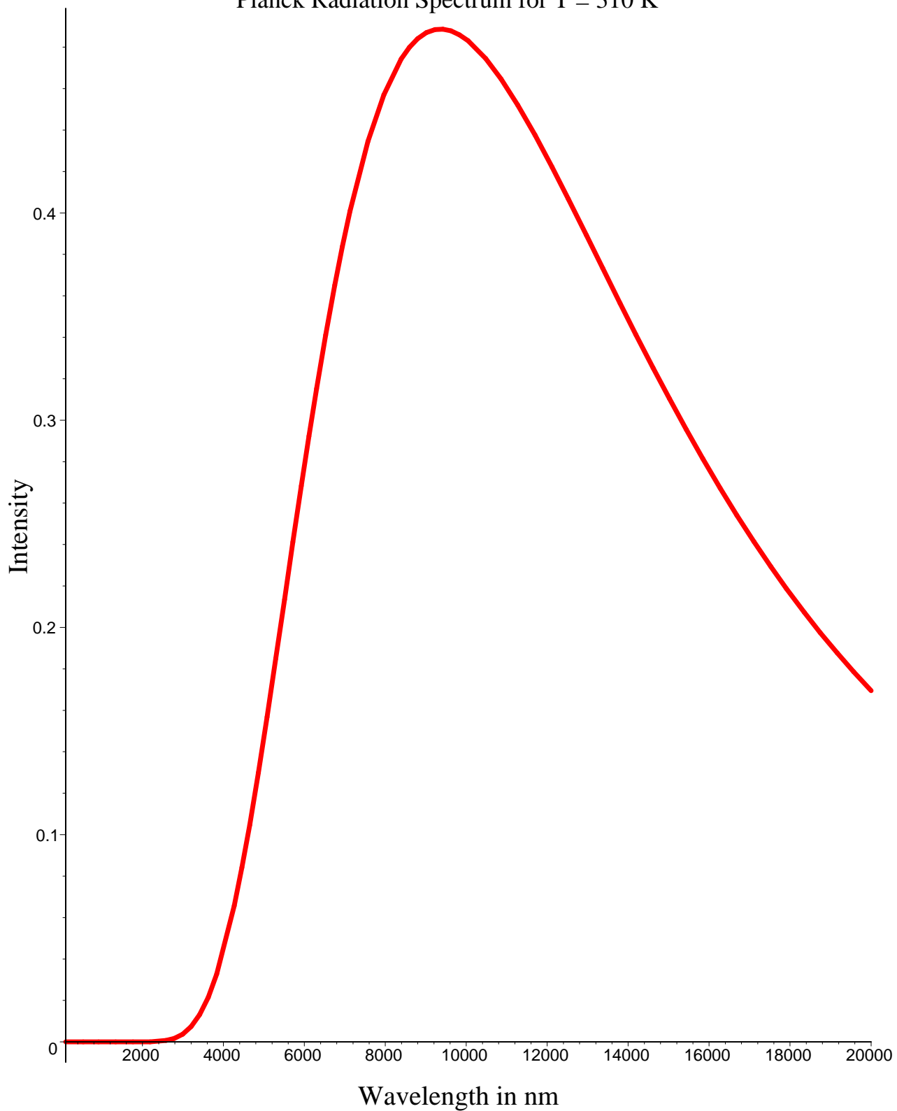
Planck Radiation Spectrum for T = 310\text{ K}
