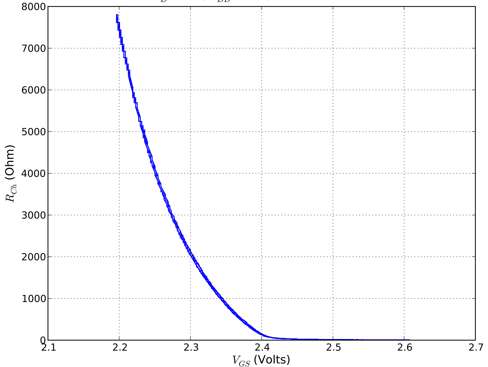
R_{Ch}(V_{GS}) for BS170 n-Channel Enhancement Mode MOSFET, R_D = 2k\Omega , V_{DD} = 10 V, 3 kHz Sine Wave
