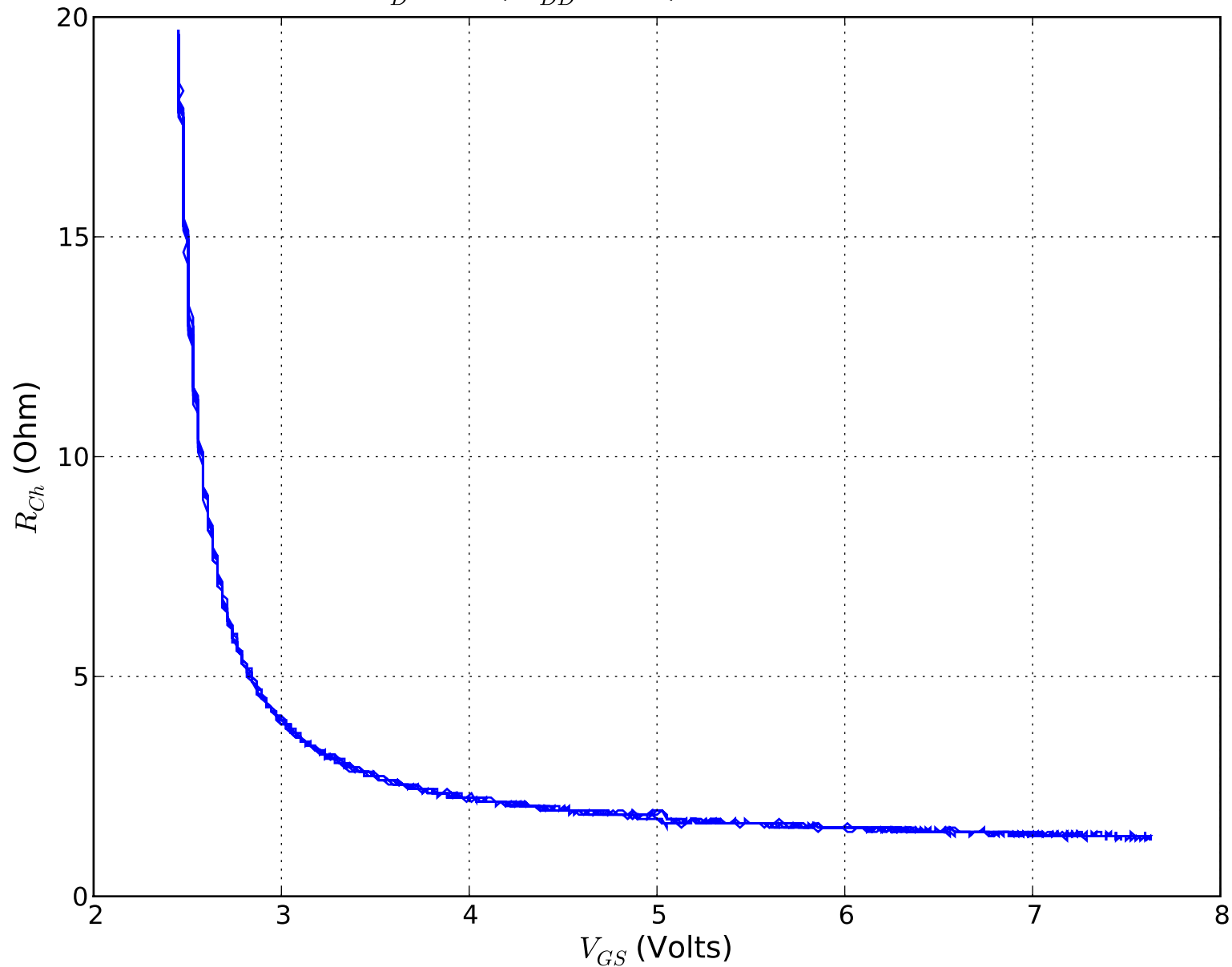
R_{Ch}(V_{GS}) for BS170 n-Channel Enhancement Mode MOSFET, R_D = 2k\Omega , V_{DD} = 10 V, 3 kHz Sine Wave
