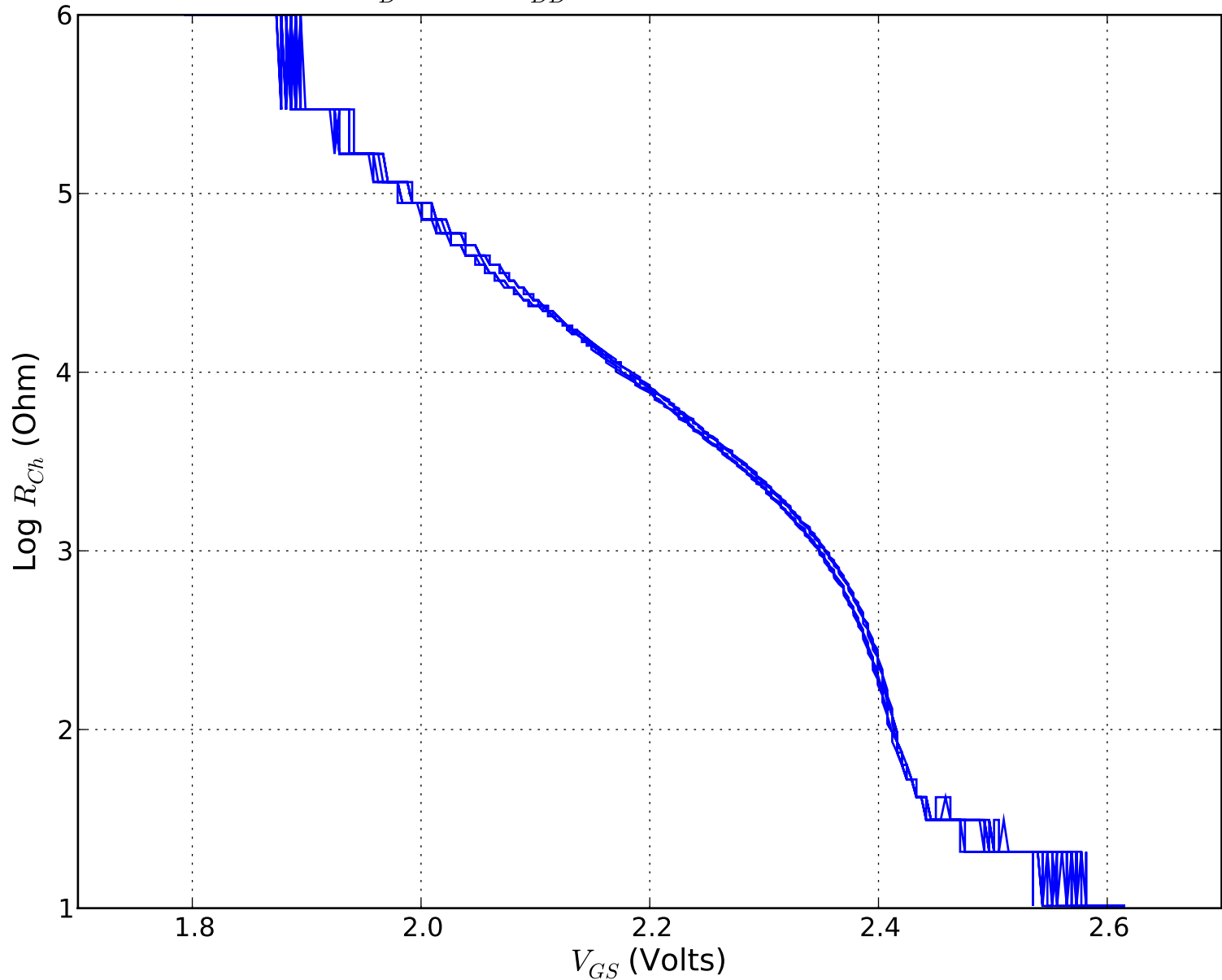
R_{Ch}(V_{GS}) for BS170 n-Channel Enhancement Mode MOSFET, R_D = 2k\Omega , V_{DD} = 10 V, 3 kHz Sine Wave
