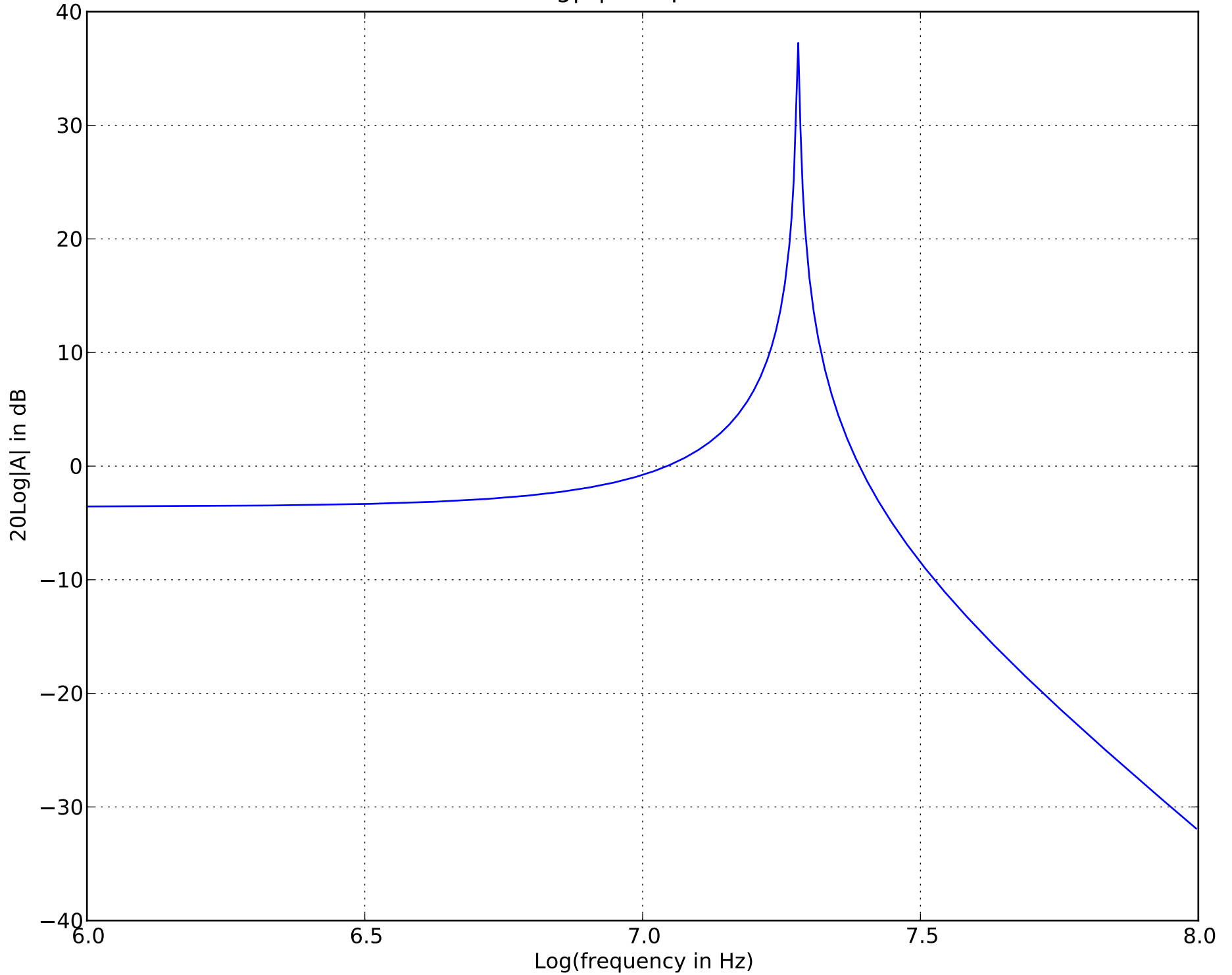
20Log|A| : Colpitts Tank
