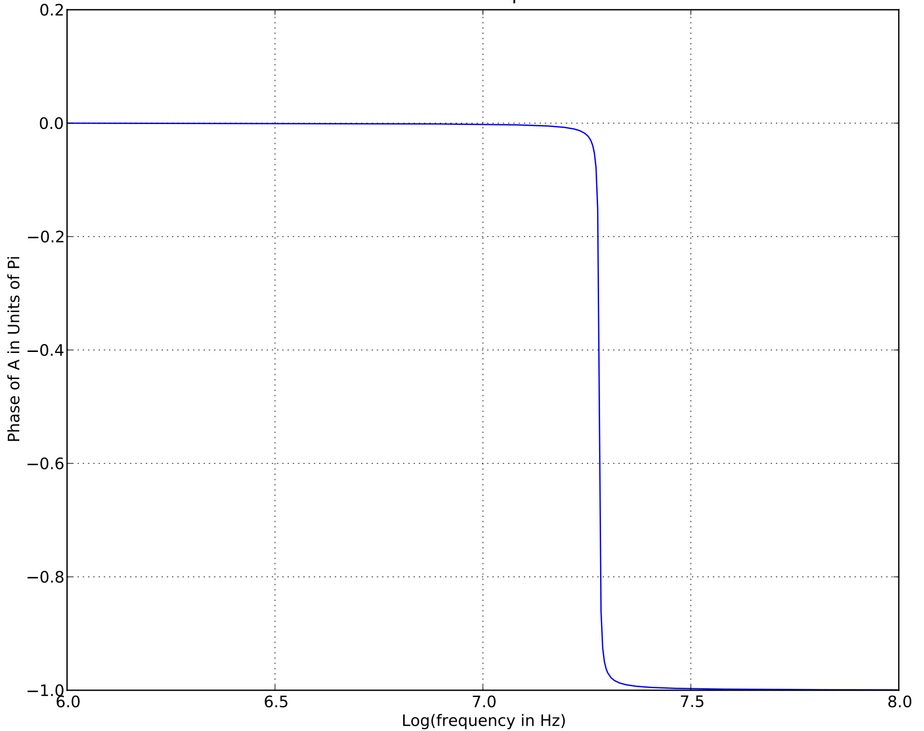
Phase of A : Colpitts Tank
