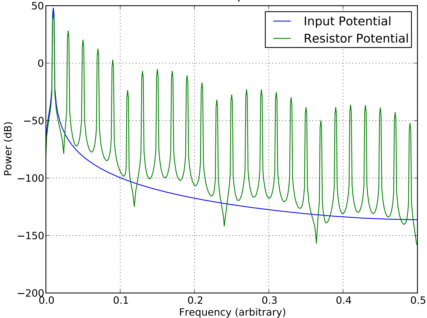
Parallel Opposite Diodes in Series with a Resistor: Sinusoidal Input Power Spectra
