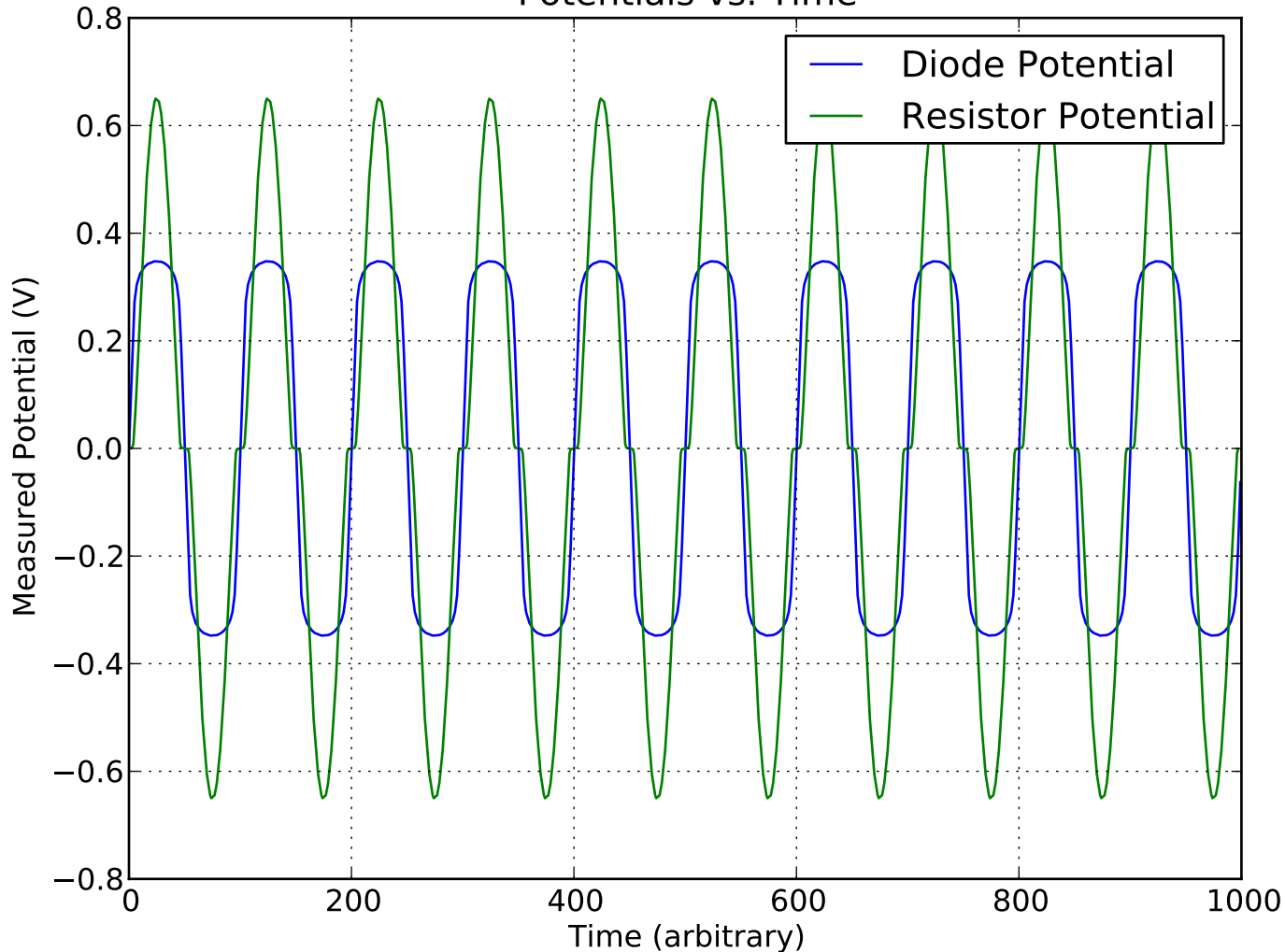
Parallel Opposite Diodes in Series with a Resistor: Sinusoidal Input Potentials vs. Time
