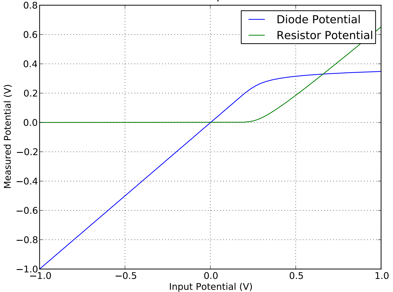
Single Diode in Series with a Resistor: DC Input Measured vs. Input Potentials
