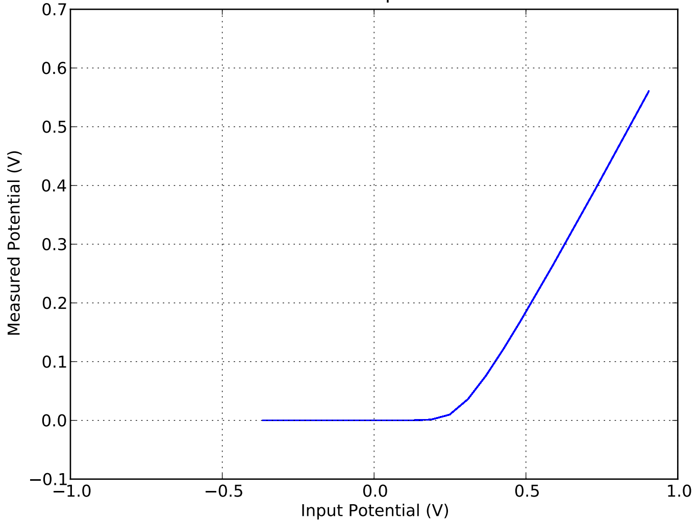
Single Diode in Series with a Resistor: Sinusoidal Input Measured vs. Input Potentials
