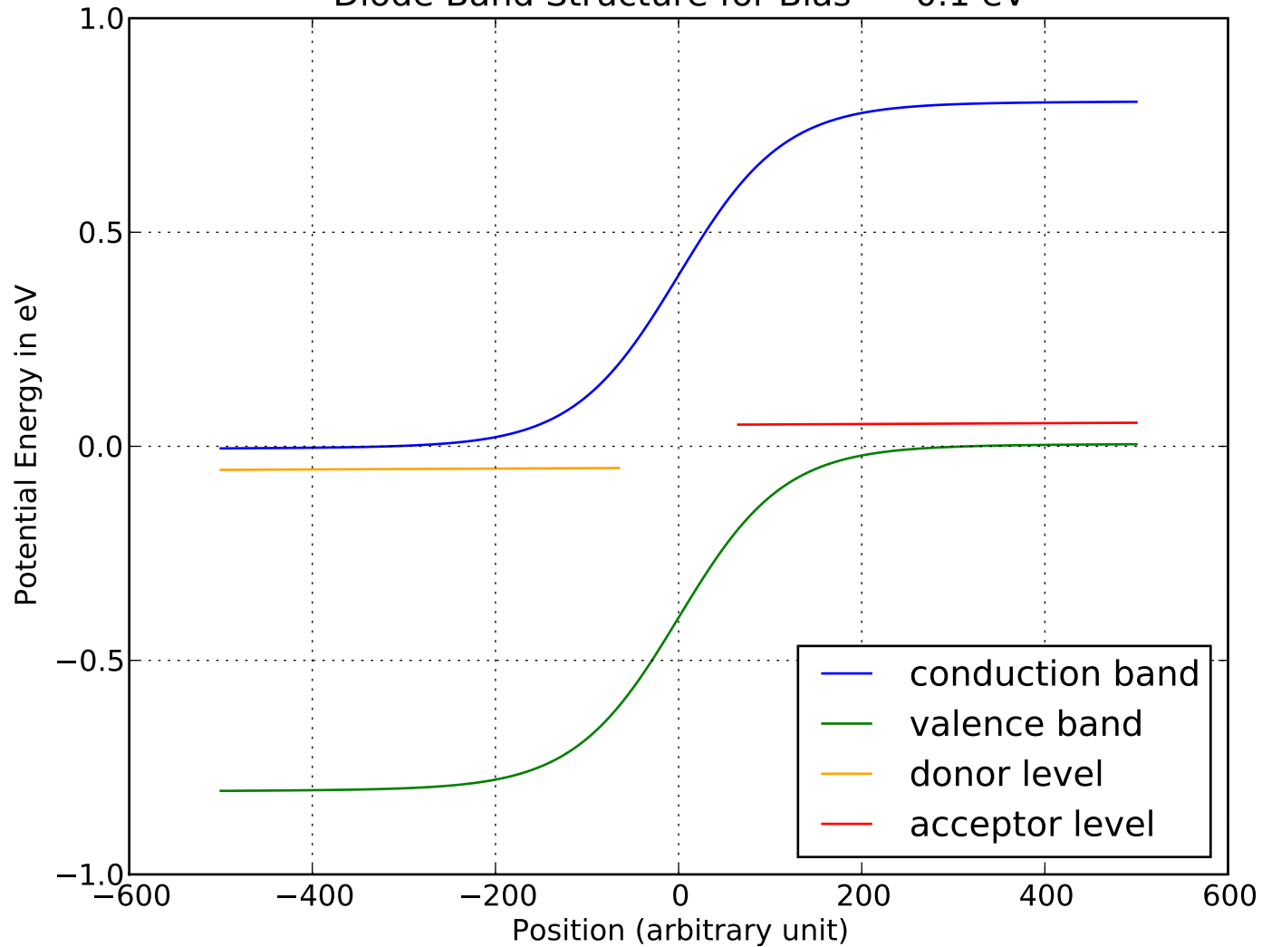
Diode Band Structure for Bias = -0.1 eV
