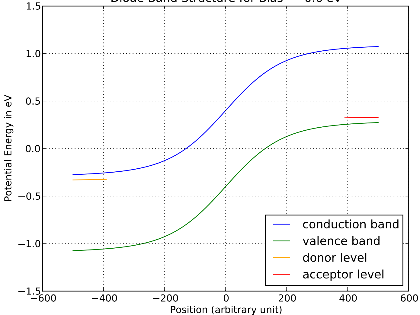
Diode Band Structure for Bias = -0.6 eV
