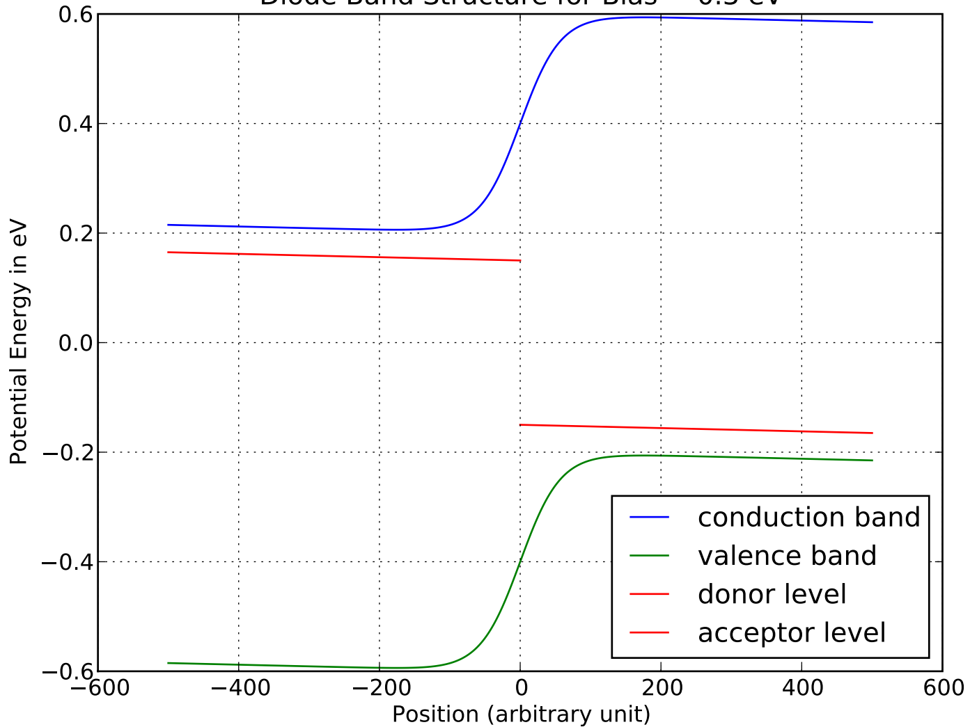
Diode Band Structure for Bias = 0.3 eV
