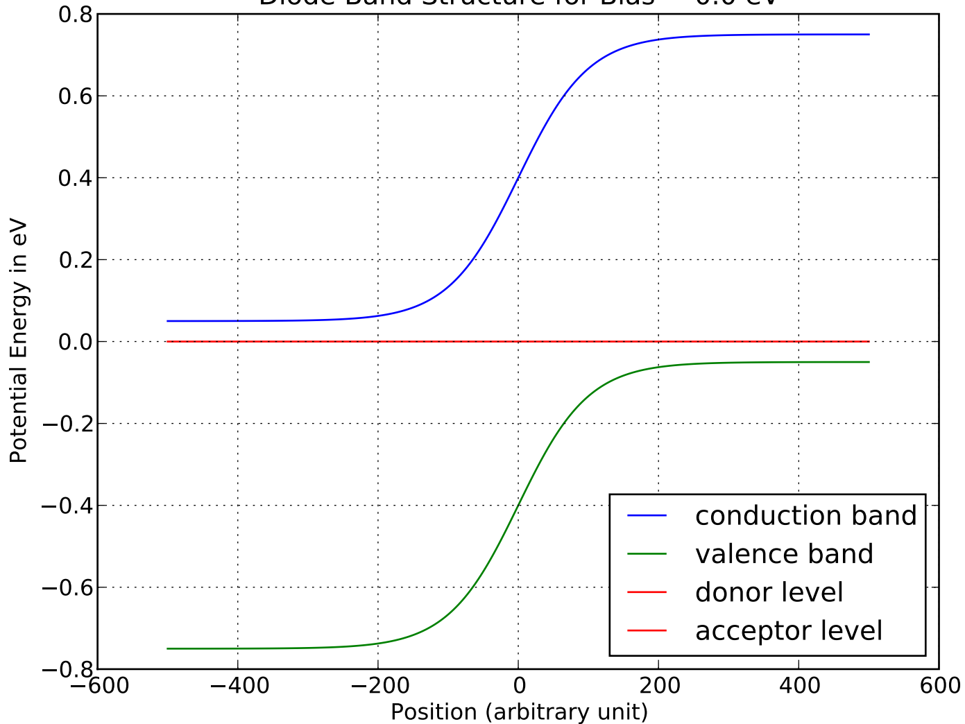
Diode Band Structure for Bias = 0.0 eV
