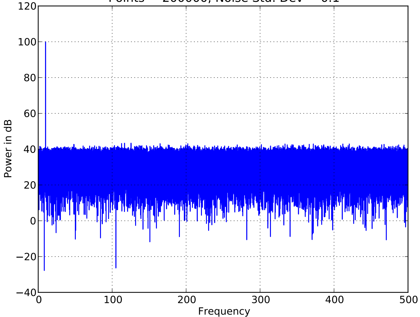
Power Spectrum of Noisy Sinewave: \lambda=0.1 , Amplitude = 1.0 Points = 200000, Noise Std. Dev = 0.1
