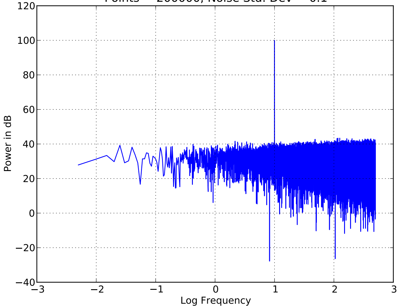
Power Spectrum of Noisy Sinewave: \lambda=0.1 , Amplitude = 1.0 Points = 200000, Noise Std. Dev = 0.1
