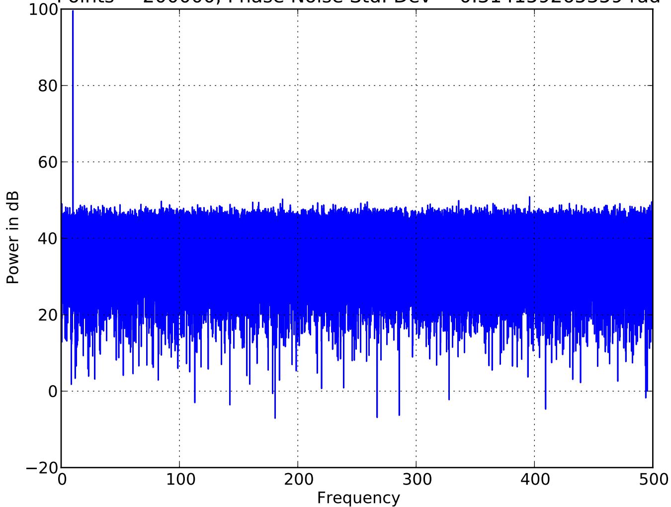
Power Spectrum of Phase-Noisy Sinewave: \lambda=0.1 , Amplitude = 1.0 Points = 200000, Phase Noise Std. Dev = 0.314159265359 rad
