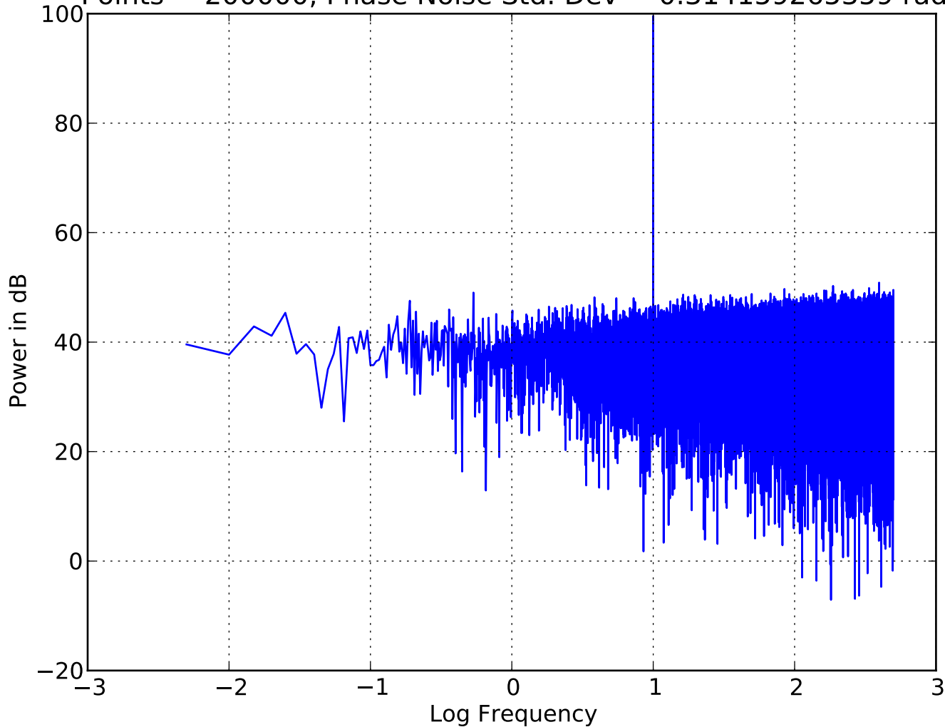
Power Spectrum of Phase-Noisy Sinewave: \lambda=0.1 , Amplitude = 1.0 Points = 200000, Phase Noise Std. Dev = 0.314159265359 rad
