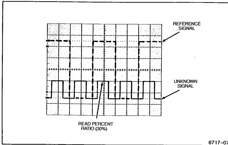
Figure 3-4. Determining voltage ratio.
