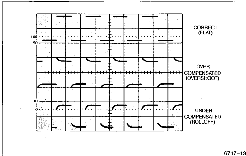
Figure 4-1. Probe compensation.
