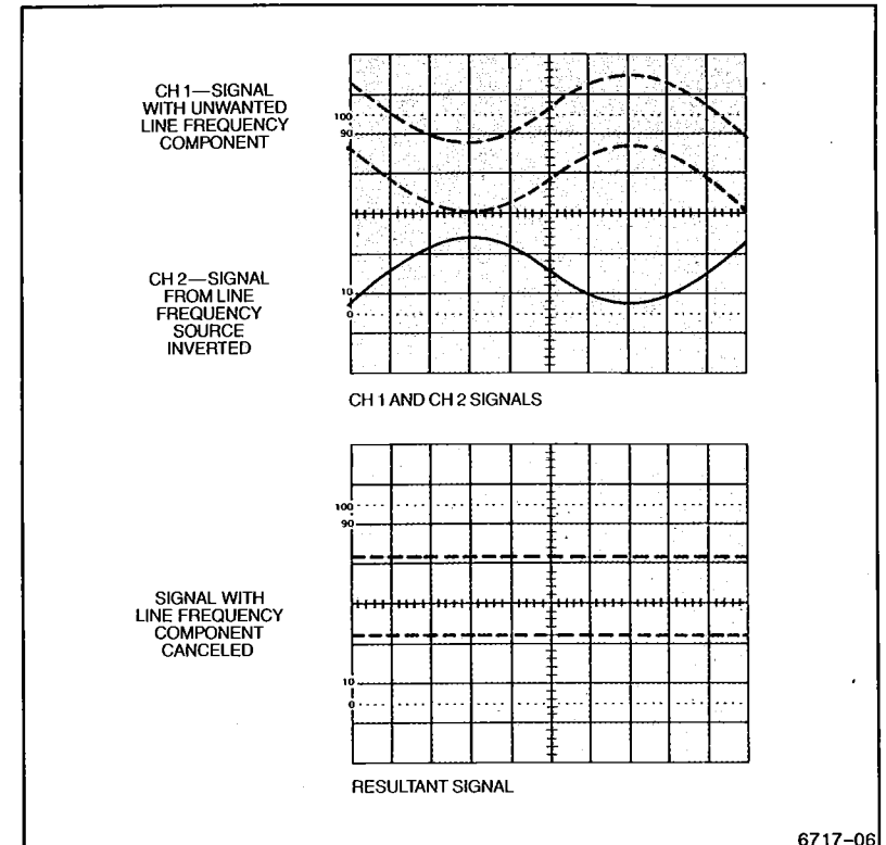
Figure 3-3. Common-mode rejection.
