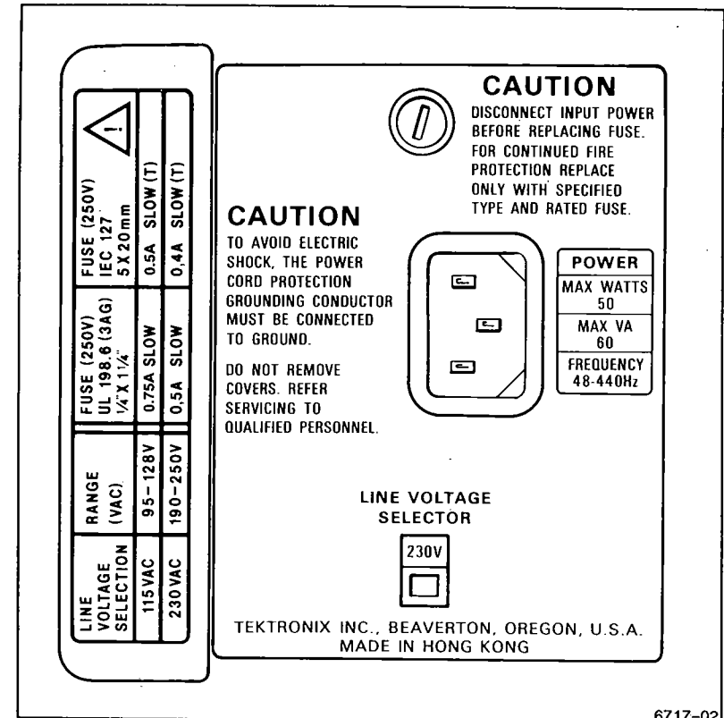
Figure 1-1. Voltage selector switch, fuse, and power-cord receptacle.
