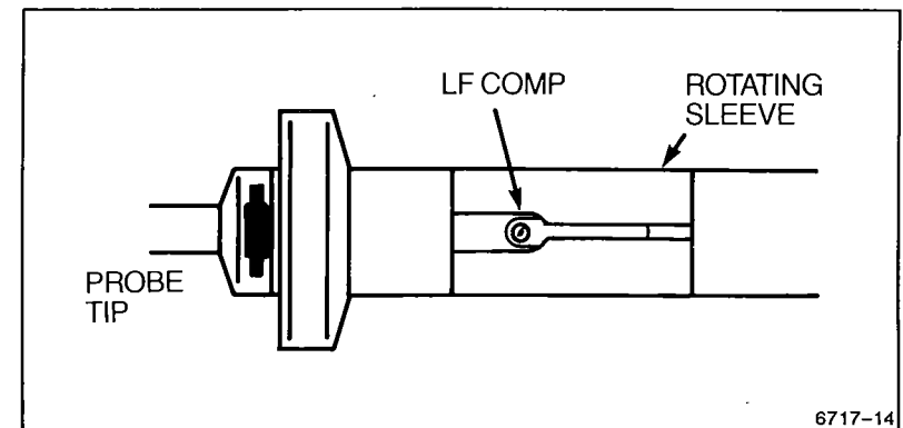
Figure 4-2. Locating the low-frequency compensation adjustment.
