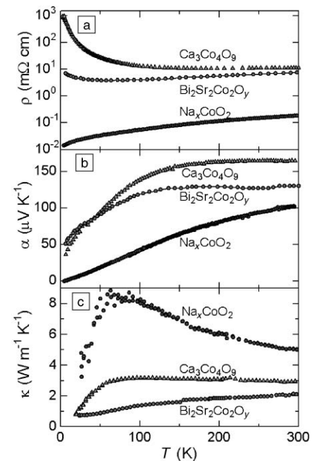
Figure 3. (a) Temperature-dependence of in-plane resistivity \rho , (b) Seebeck coefficient \alpha , and (c) thermal conductivity \kappa of the three Co oxides shown in Figure 2.
