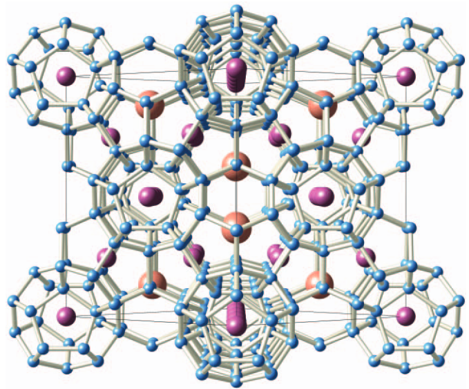
Figure 3. Crystal structure of the Type II clathrate. Framework atoms are shown in blue, guest atoms inside the tetrakaidecahedra are orange, and guest atoms inside the pentagonal dodecahedra are purple.
