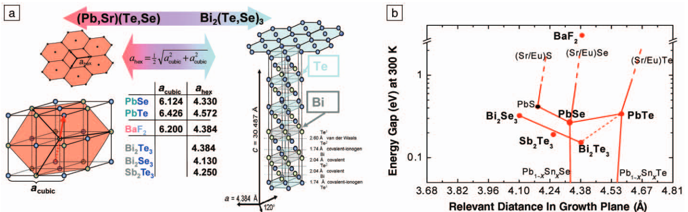
Figure 2. (a) Crystallographic data for IV-VI and V-VI compounds, highlighting the structural relationship between both material systems. (b) Epitaxial map of semiconductor materials (at room temperature) that could be suitable in combination with \text{Bi}_2\text{Te}_3 , based on their relevant atomic distance with respect to the a -plane of \text{Bi}_2\text{Te}_3 .
