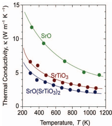
Figure 6. Thermal conductivity versus temperature for STO-327 [SrO(SrTiO 3 ) 2 ] compared with STO39 (SrTiO 3 ) and SrO. 40
