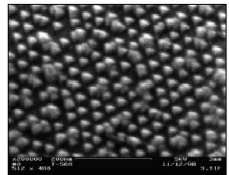
Figure 4. Quantum dot structures in the \text{PbTe}/\text{PbSeTe} system. 42
