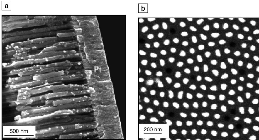
Figure 5. Scanning electron micrographs of \text{Bi}_2\text{Te}_{3-x}\text{Se}_x , showing an array of 50-nm-diameter templated nanowires: (a) cross section; (b) bottom view after removal of Pt electrode. Taken from Figure 6 in Reference 25.
