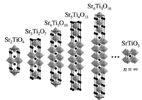
Figure 5. Crystal structures of the Ruddlesden-Popper homologous series. 36 Each octahedron consists of TiO 6 . The solid black dots denote Sr ions.
