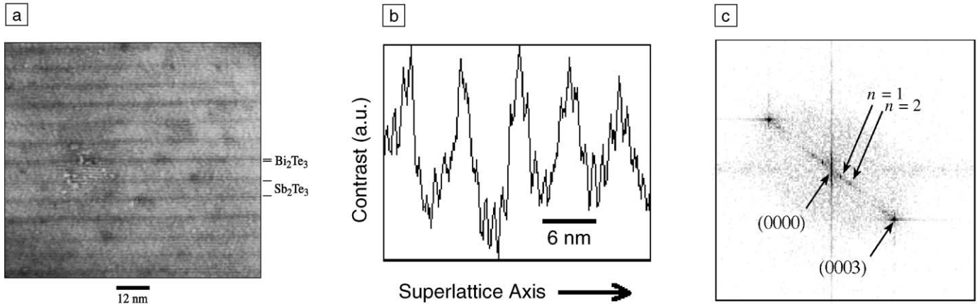
Figure 3. (a) Transmission electron micrograph of a \text{Bi}_2\text{Te}_3/\text{Sb}_2\text{Te}_3 ( 10 \text{ \AA}/50 \text{ \AA} ) superlattice. (b) Image contrast oscillations through the superlattice. (c) Fast Fourier transform of the image in (a), showing the superlattice reflections of order n . 22
