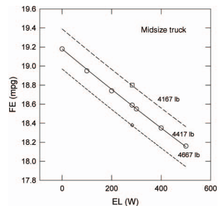
Figure 6. Dependence of fuel economy (FE) in miles per gallon (mpg) on electrical load (EL) at the alternator for a representative midsize truck at various weights. The symbols are data simulated by Overdrive, and the lines are guides for the eye.
